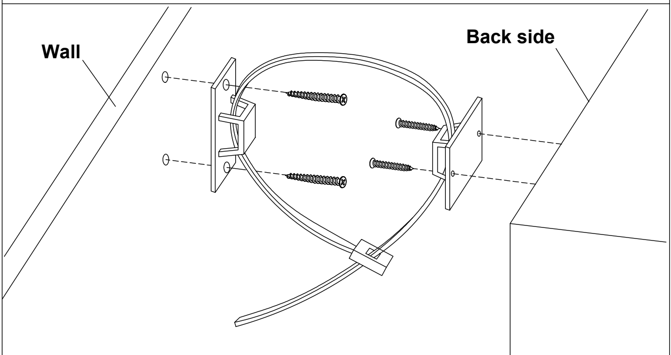
Mounting Plate x 2
